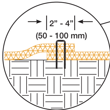
Detail 3A "Overlap"
